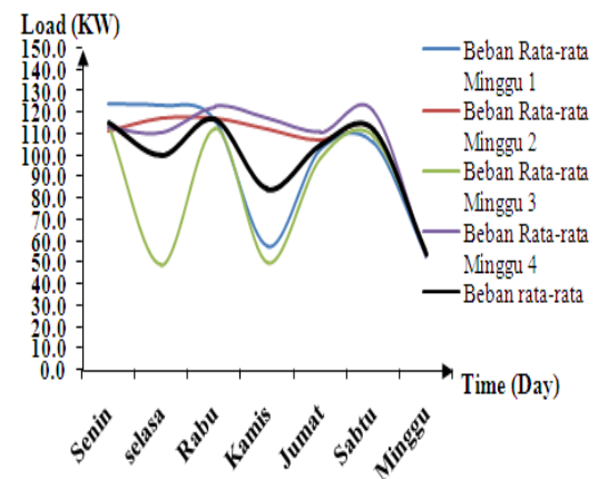
Gambar.6 Kurva Beban Rata – rata harian selama 1 bulan
