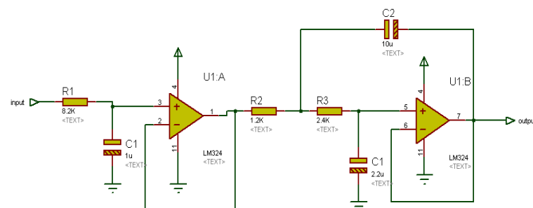
Gambar 3.5 Rancangan LPF butterworth sallen key orde 3
