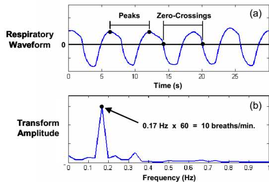
Gambar 1.3 The two primary methods of assessing respiratory waveforms: (a) measuring individual breathing cycle intervals and (b) performing spectral analysis (S, William. 2006)
