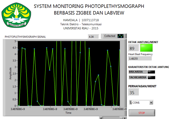
Gambar 3.4 Sistem monitoring photoplethysmograph berbasis zigbee dan labview
