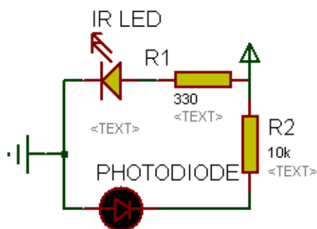
Gambar 2.2 Rangkaian sensor photoplethysmograph
