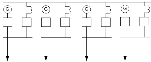
Gambar 2.4 Gambar 2.5 Sistem star bus (Irfan, 2007)
