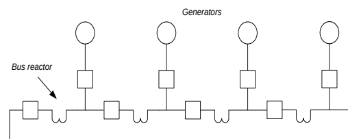
Gambar 2.3 Sistem ring bus (Skrotzki, 1954: 436)
