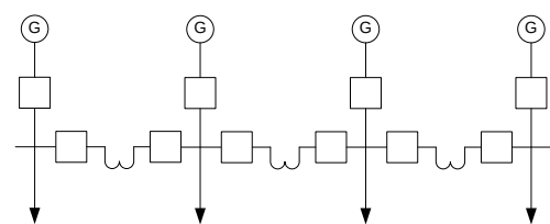
Gambar 2.2 Sistem Straight bus (Irfan, 2007)
