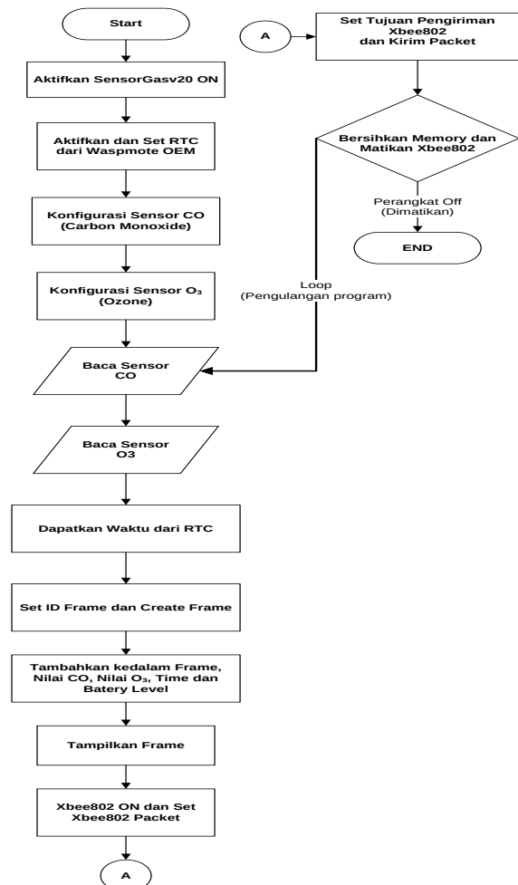
Gambar 8 Flowchart Pemrograman Wasmote Libelium OEM
