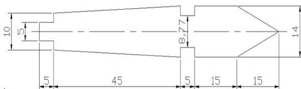
Gambar 2 Dead center 2D
