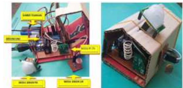
Gambar 3.8 Hasil Rangkaian Transmitter
