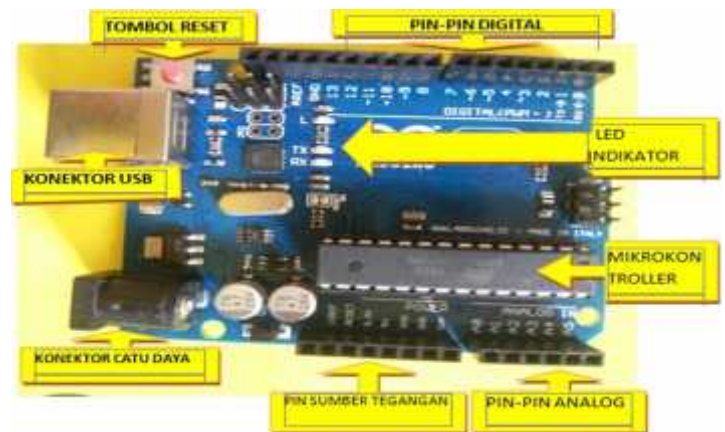
Gambar 2.1 Board Arduino UNO
