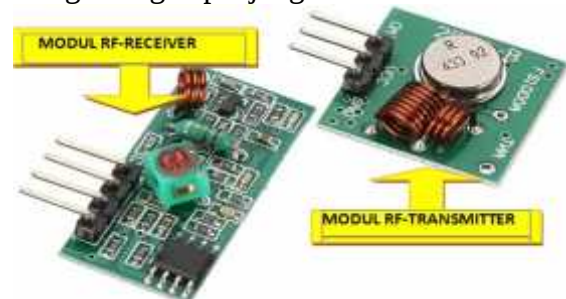
Gambar 2.2 Modul RF 433MHz
