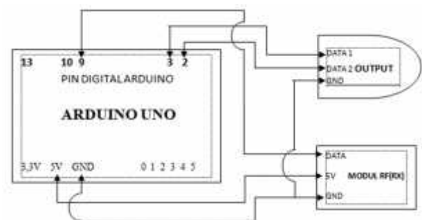
Gambar 3.9 Desain Rangkaian Receiver
