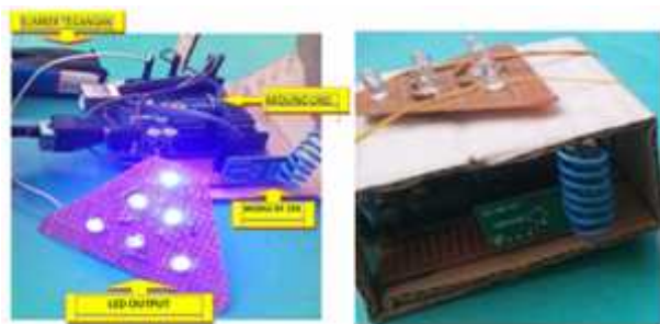
Gambar 3.10 Hasil Rangkaian Receiver
