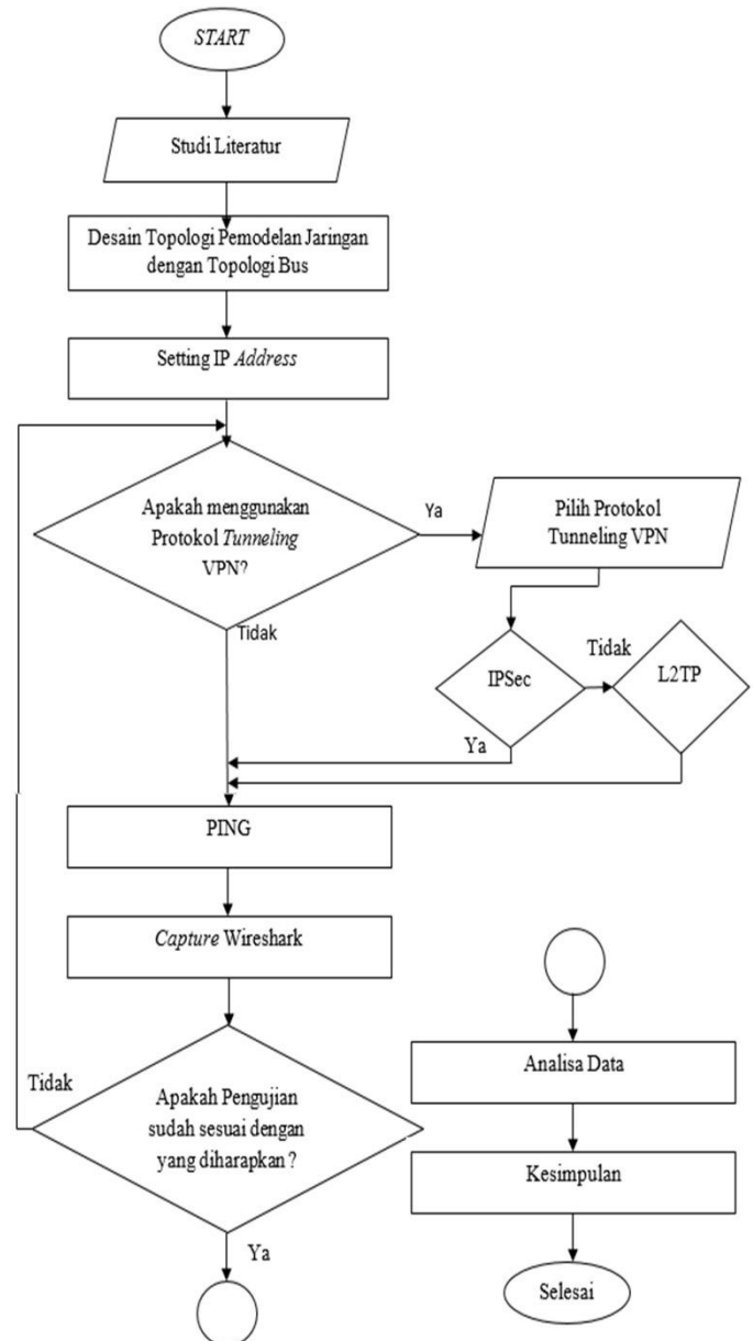
Gambar 1. Flowchart Penelitian
