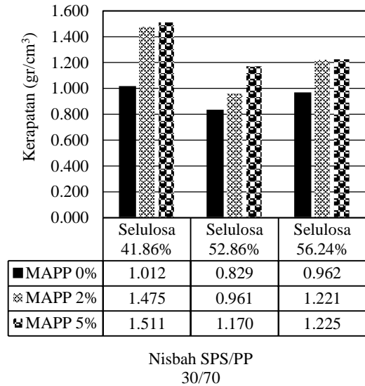
Gambar 3 Nilai Rata-rata Kerapatan Material WPC rasio SPS/PP (30/70)
