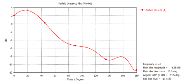
Gambar 3.6 Gain antenna
