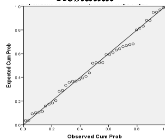
Gambar 1 Normal Probability Standardized Residual
