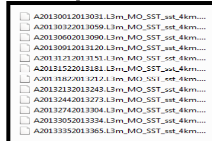
Gambar 4.Data Citra Satelit Aqua MODIS level 3 resolusi 4 km.
